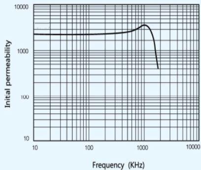
Initial Permeability VS Frequency
