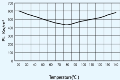
Power loss VS Temperature 100KHz 200mT
