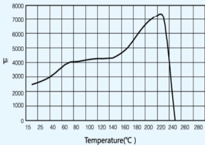
Permeability VS Temperature
