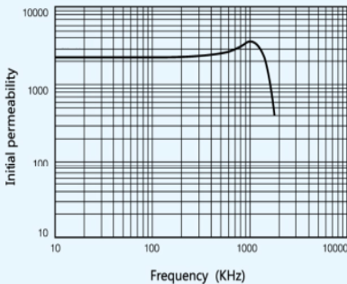
Initial Permeability VS Frequency
