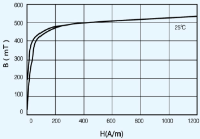
B-H
