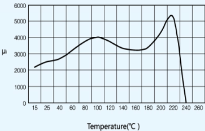
Permeability VS Temperature
