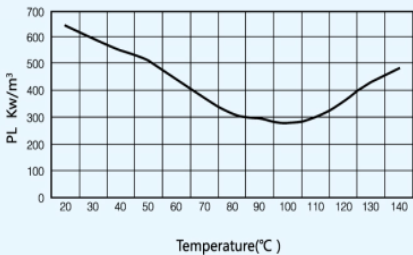
Power loss VS Temperature 100KHz 200mT
